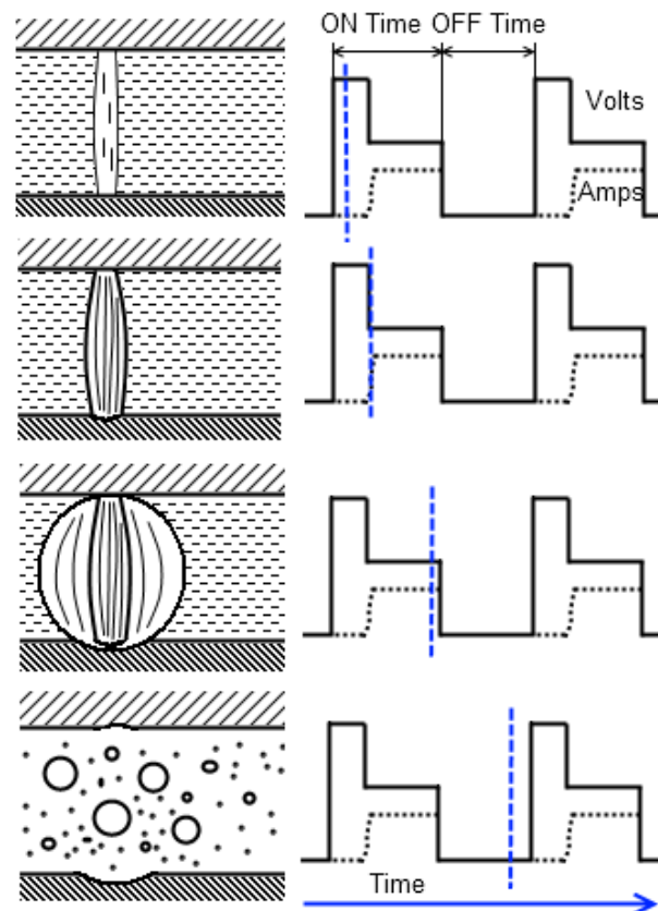
Fig. 1. Diagram of the spark material removal process.
